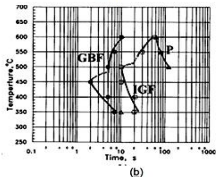
Figure 1. Initial Stage Of TTT Diagram: (a) V- Steel (b) V – Ti Steel; Closed Circles - Grain Boundary Ferrite (GBF); Open Squares – Intra-Granular Ferrite (IGF), Open Triangles – Bainitic Sheaves (BS); Closed Triangles – Pearlite (P).
